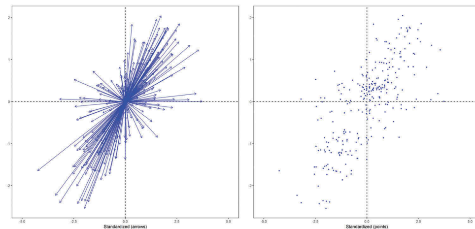
Figure 3. Standardized Moran scatterplots for 2000–2015, ECO-DEV.
