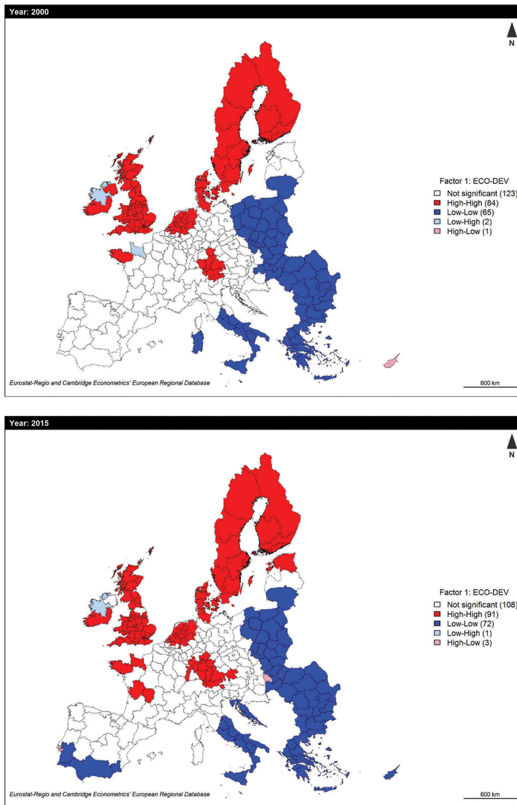
Figure 1. Local Moran clusters for 2000 and 2015 (ECO-DEV) – p -value = 0.05 with Bonferroni adjustment.
