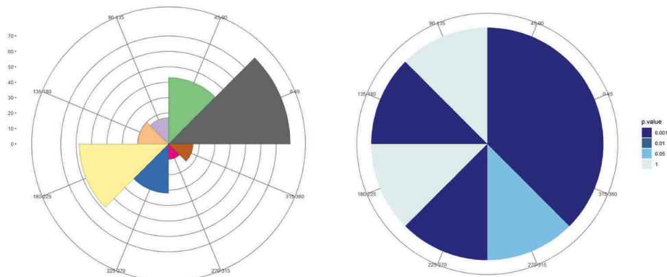
Figure 4. Rose diagram and p-values for k = 8 , ECO-DEV.
